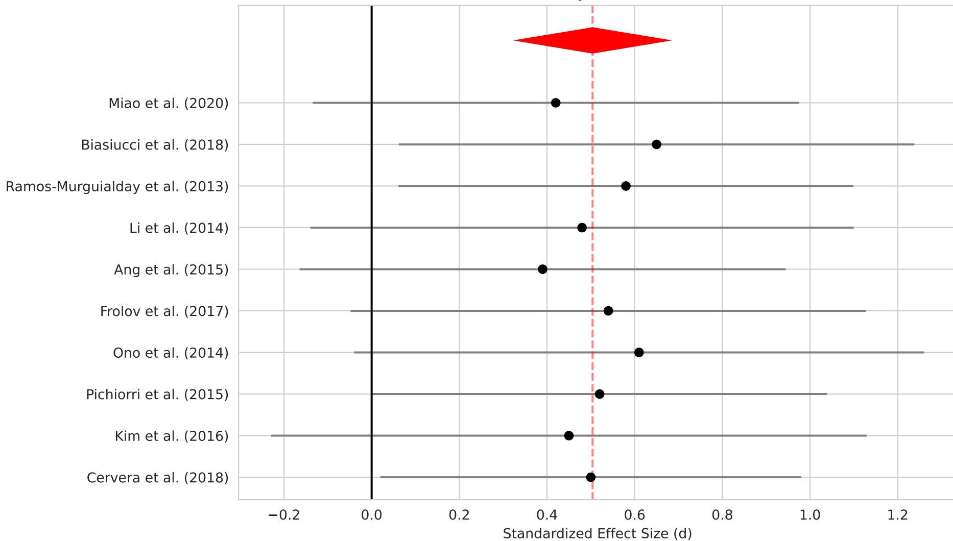
Meta-Analysis Forest Plot
