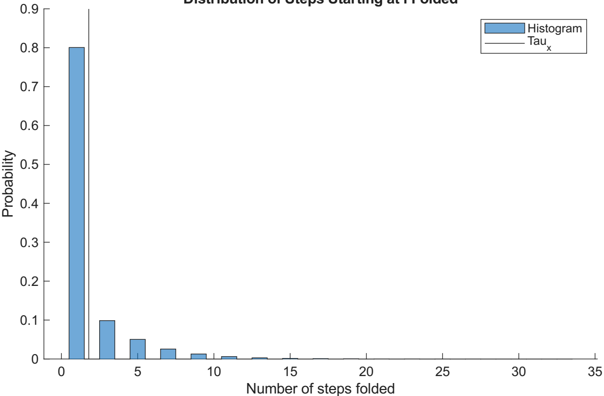
Distribution of Steps Starting at I Folded
