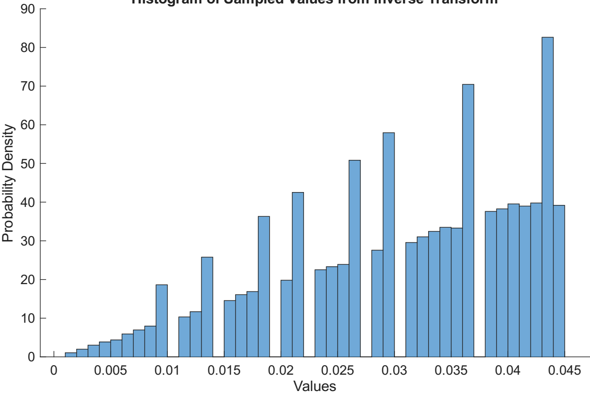
Histogram of Sampled Values from Inverse Transform
