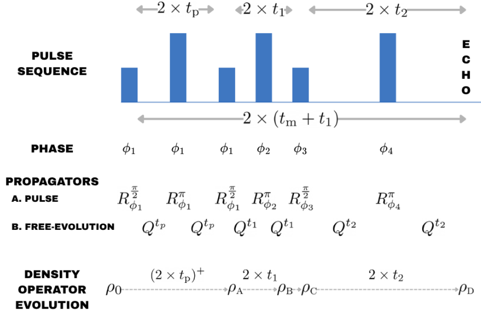
Figure 1: DQC 6-pulse sequence with the short and tall rectangles representing \pi/2 and \pi -pulses, respectively. Typically, t_m = t_p + t_2 is kept constant in an experiment, while varying t_p from 0 to t_m ( t_2 = t_m - t_p ); t_1 is kept constant as well. The pulse phases ( \phi_j ) and the propagators, for each pulse ( R ) and free-evolution ( Q ), are shown. Starting from the equilibrium density operator \rho_0 , the overall density operator expressions are derived in four stages: preparation of multiple quantum coherences ( \rho_A ), refocusing of DQC ( \rho_B ), conversion of DQC to single quantum coherence ( \rho_C ) and formation of re-focused echo ( \rho_D ).
