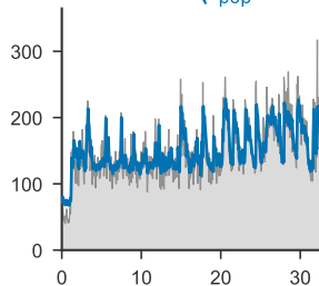
Transformer ( r_{\text{pop}} = 0.80 )
