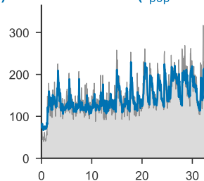
GatedDeltaNet ( r_{\text{pop}} = 0.80 )
