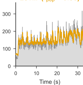
LSTM ( r_{\text{pop}} = 0.80 )
