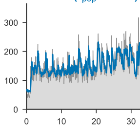
HGRN2 ( r_{\text{pop}} = 0.81 )
