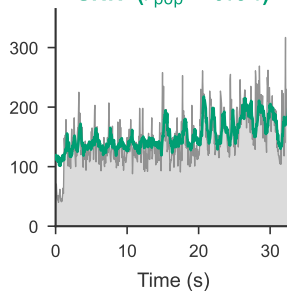
SNN ( r_{\text{pop}} = 0.64 )
