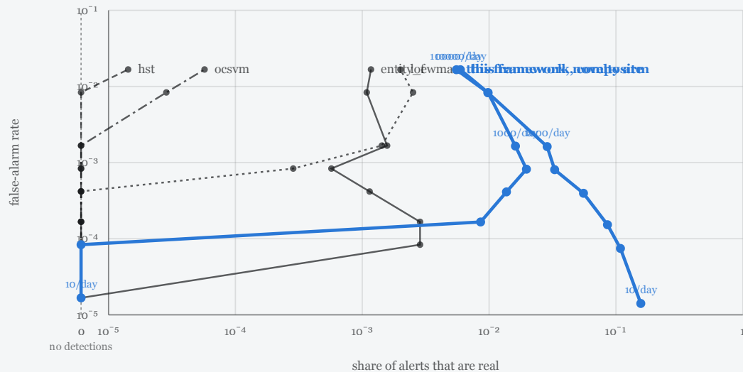
share of alerts that are real against false-alarm rate, one line per detector, across alert budgets of 10 to 10000 alerts a day
