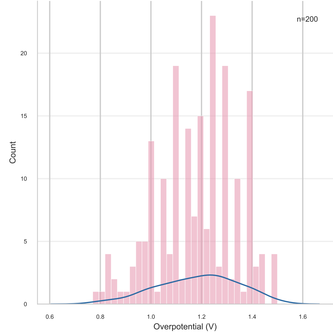
(a) Overpotential Distribution
