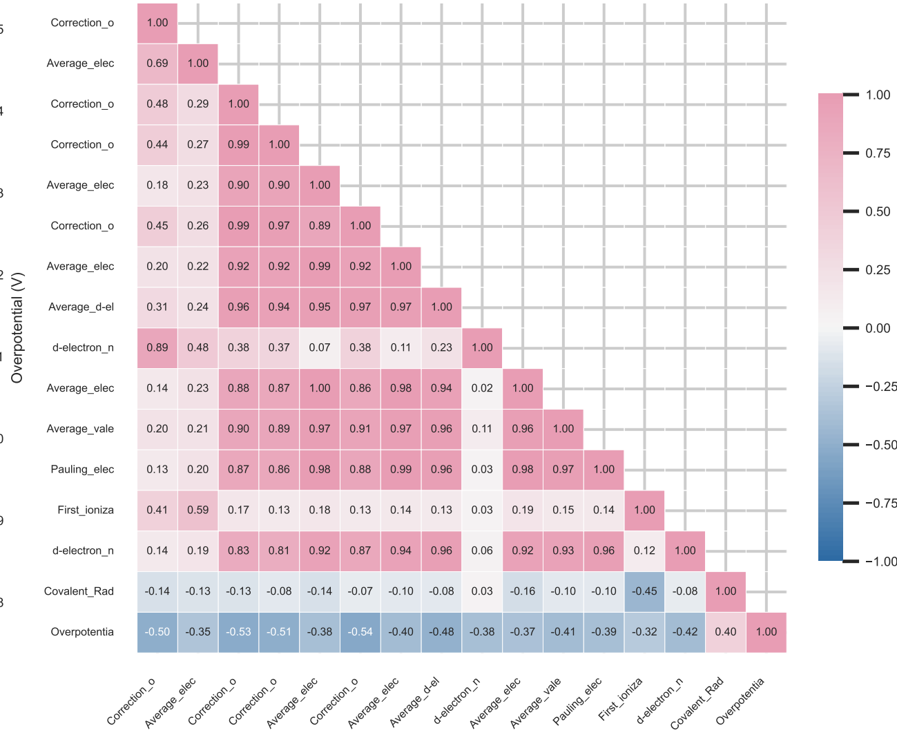
(e) Feature Correlations with Overpotential
