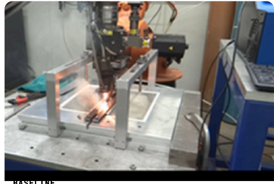
Welding without ultrasound — larger plasma plume.
