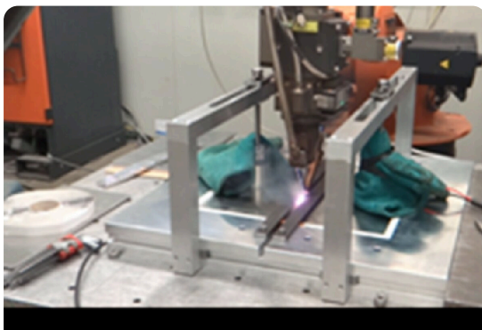
Stabilised keyhole, reduced plasma and spatter.
