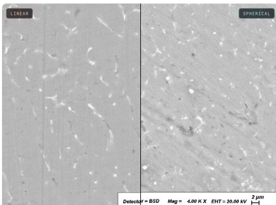
FIG. 4 – INTERMETALLICS, SEM 4000x (BSD, 20 KV)
