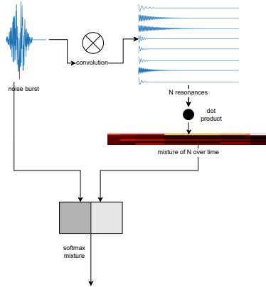
Fig. 3: Decoder Block
