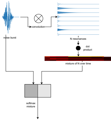
Fig. 3: Decoder Block
