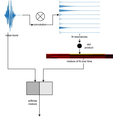
Fig. 3: Decoder Block
