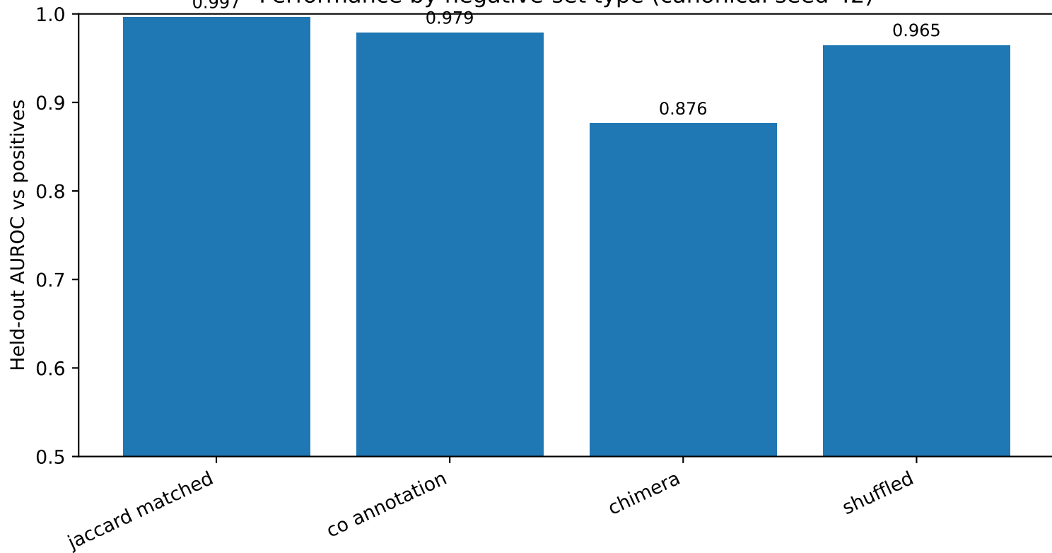
Performance by negative-set type (canonical seed 42)
