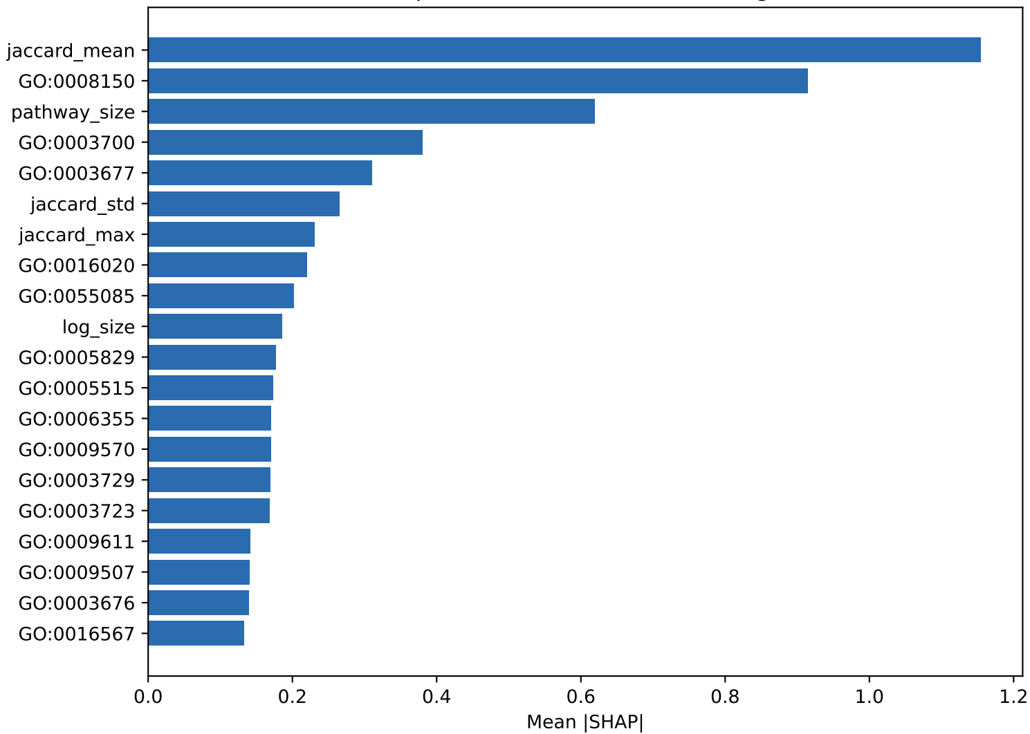
Top SHAP features (no embedding)
