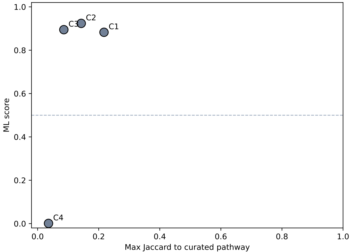
Candidate scoring
