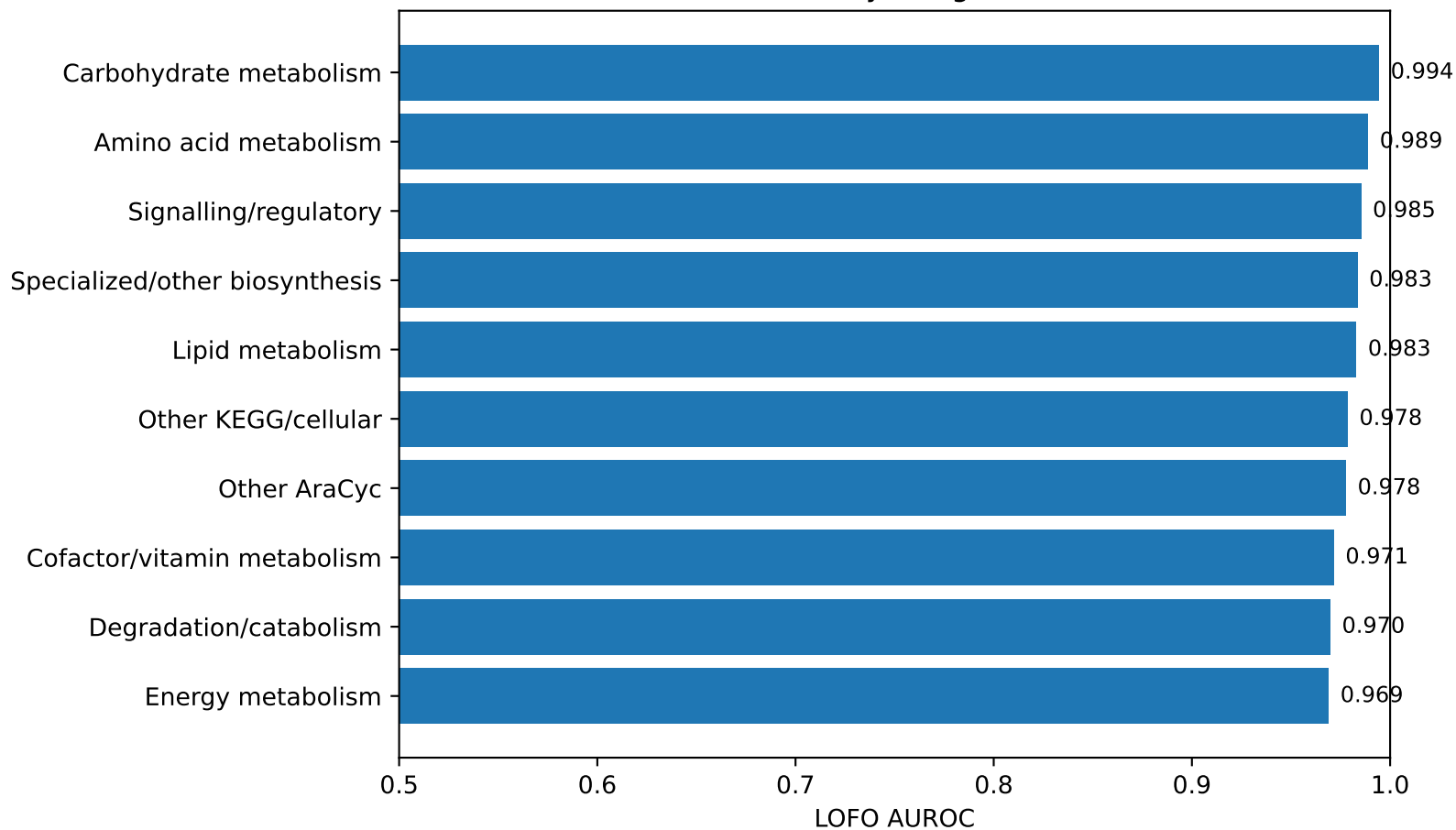
Leave-one-family-out generalisation
