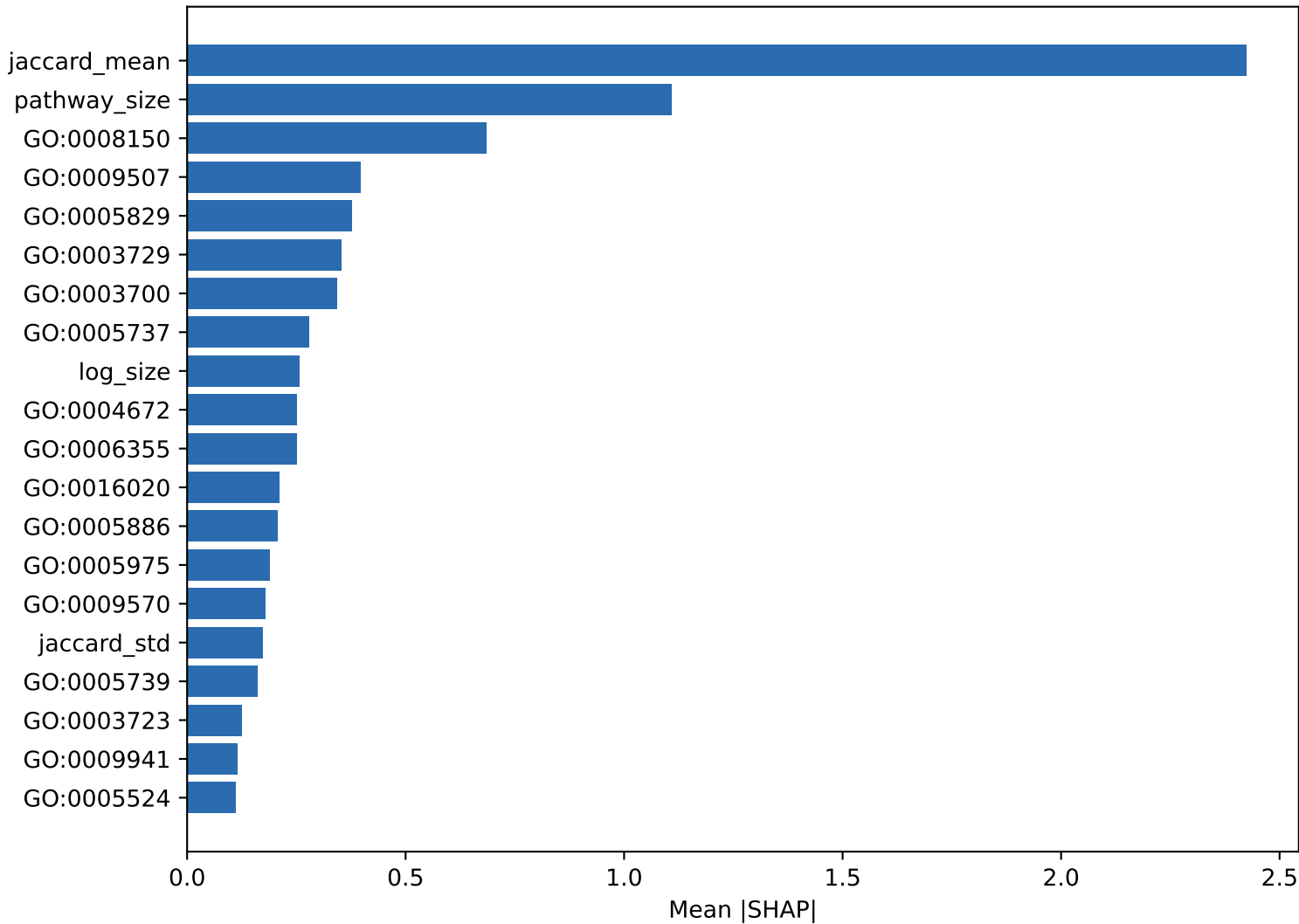
Top SHAP features (no embedding)
