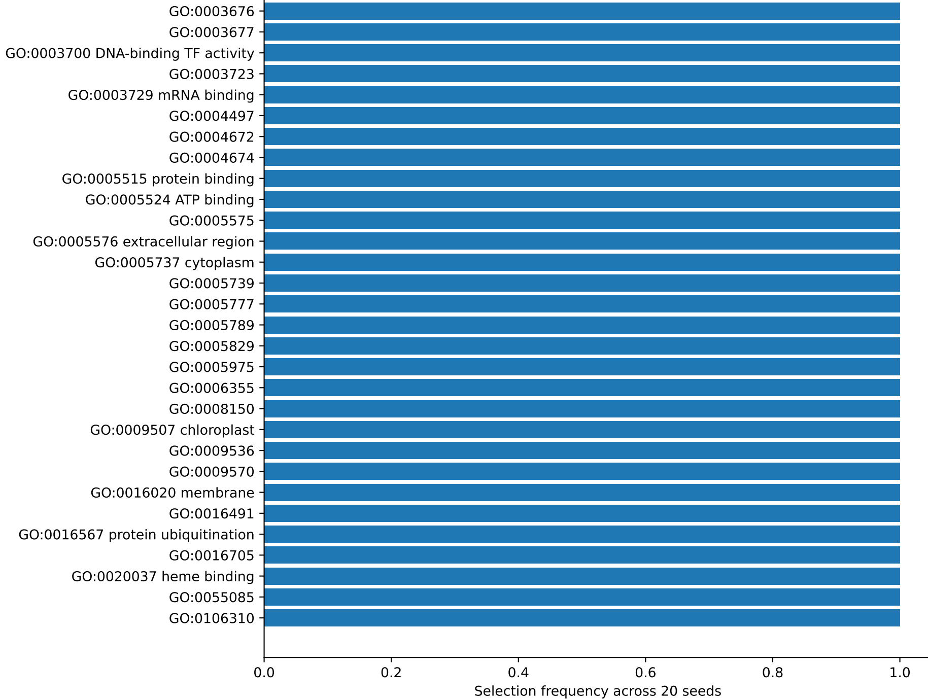
Most stable GO frequency features
