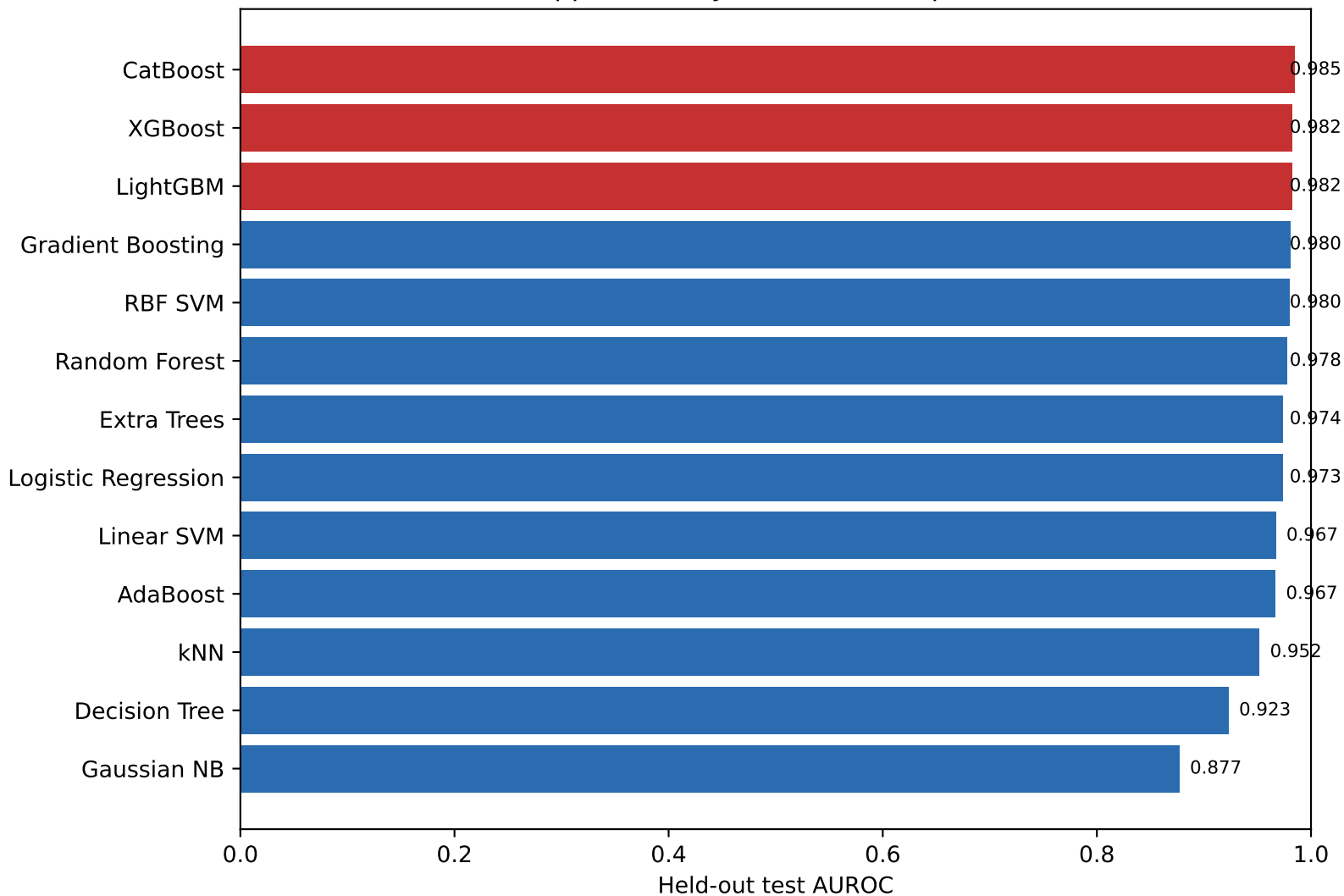
Supplementary 13-model comparison
