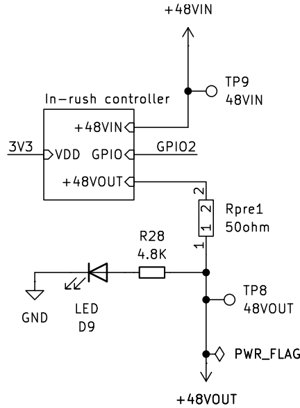
Figure 1: Detail of the solid-state pre-charge topology. The 50\ \Omega resistor R_{PRE1} dominates the branch impedance, physically limiting the maximum current to 0.96 A regardless of the state of the LM5069 controller.
