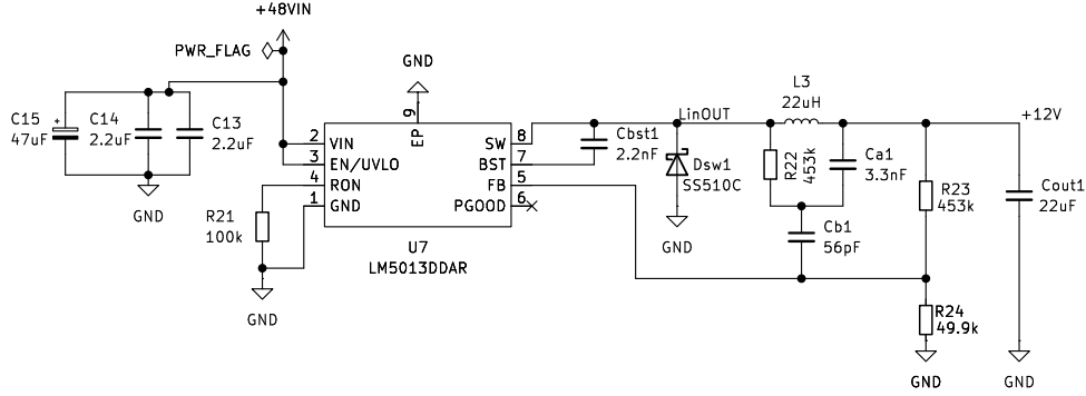
Figure 4: Topology of the LM5013 step-down converter. The main components are: the 22\ \mu\text{H} inductor L_3 , the bypass diode Dsw1 (SS510C), and the R_{23}/R_{24} feedback network for precise regulation of the 12 V output.
