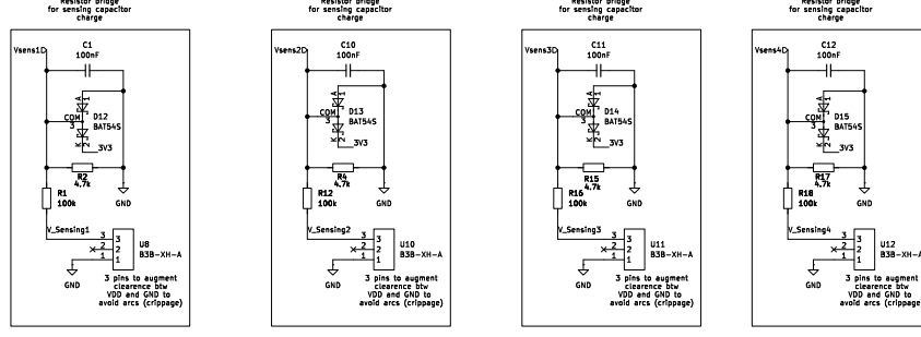
Figure 3: Schematic diagram of the V\_Sensing modules used by the ESP32 to read the bus voltage. Note the resistor dividers connected to the BAT54S diodes, which are essential for protecting the microcontroller’s ADC inputs from transient overvoltages.
