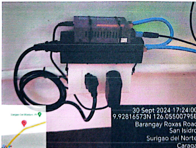
Media Converter and POE Injector
