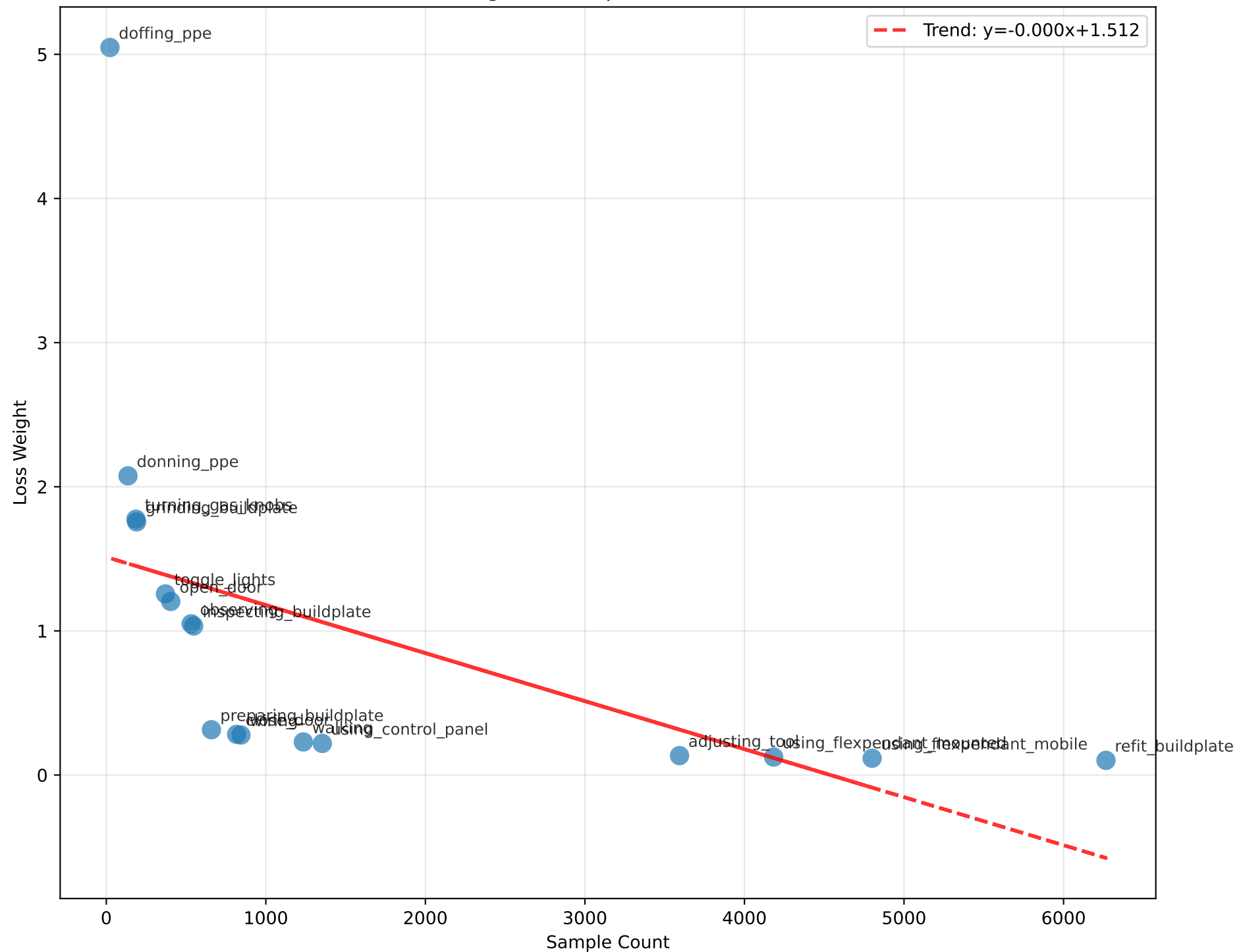
Class Weight vs Sample Count Correlation
