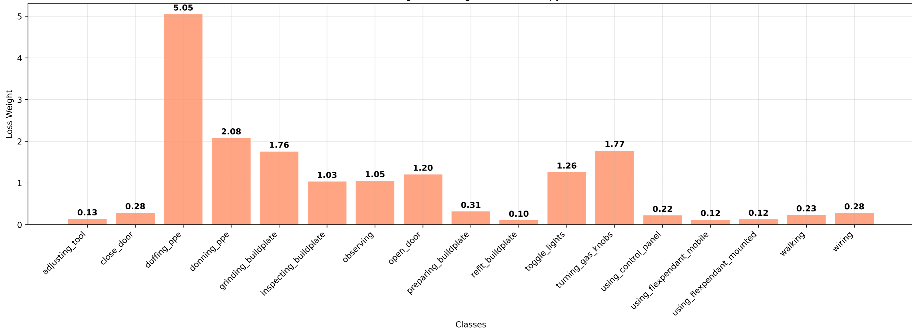
Class Weights for Weighted CrossEntropyLoss
