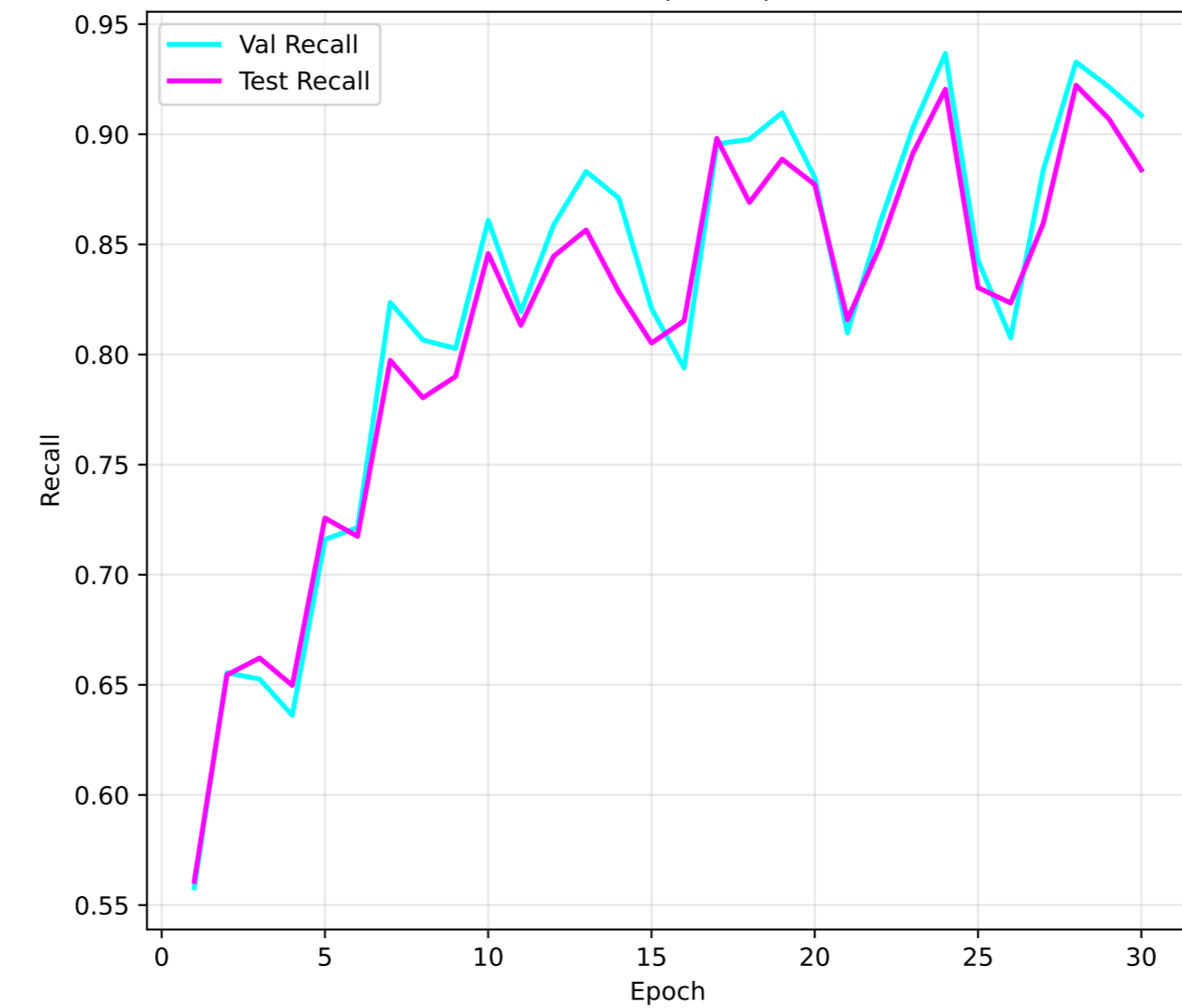
Recall (Macro)
