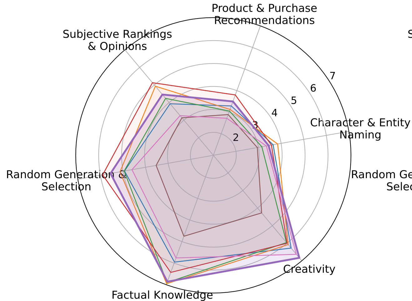
LLaDA-8B-Instruct
