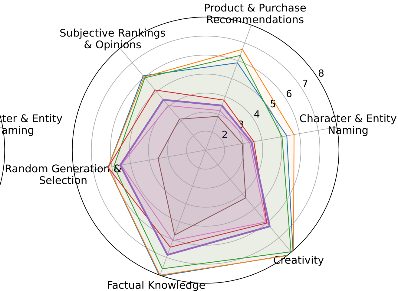
TraDo-8B-Instruct
