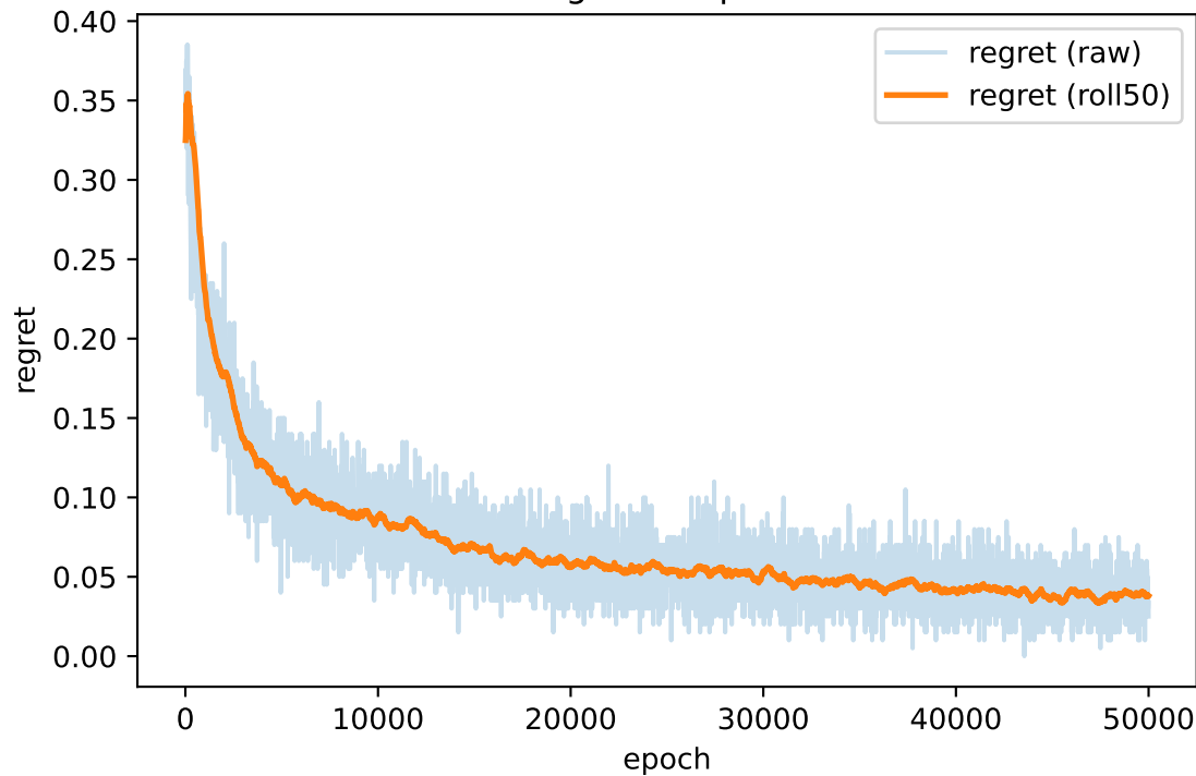
regret vs epoch
