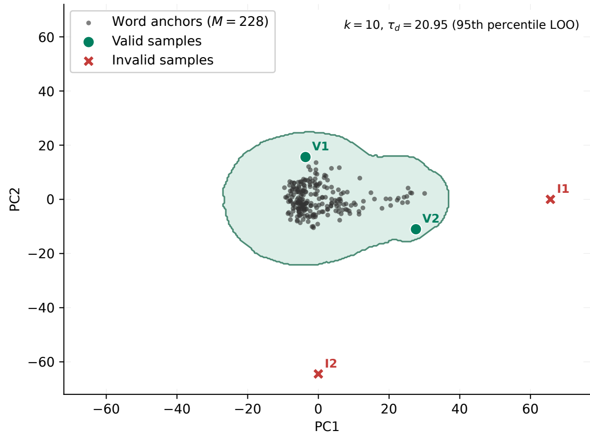
kNN validity region \mathcal{M} (PC1--PC2 slice)
