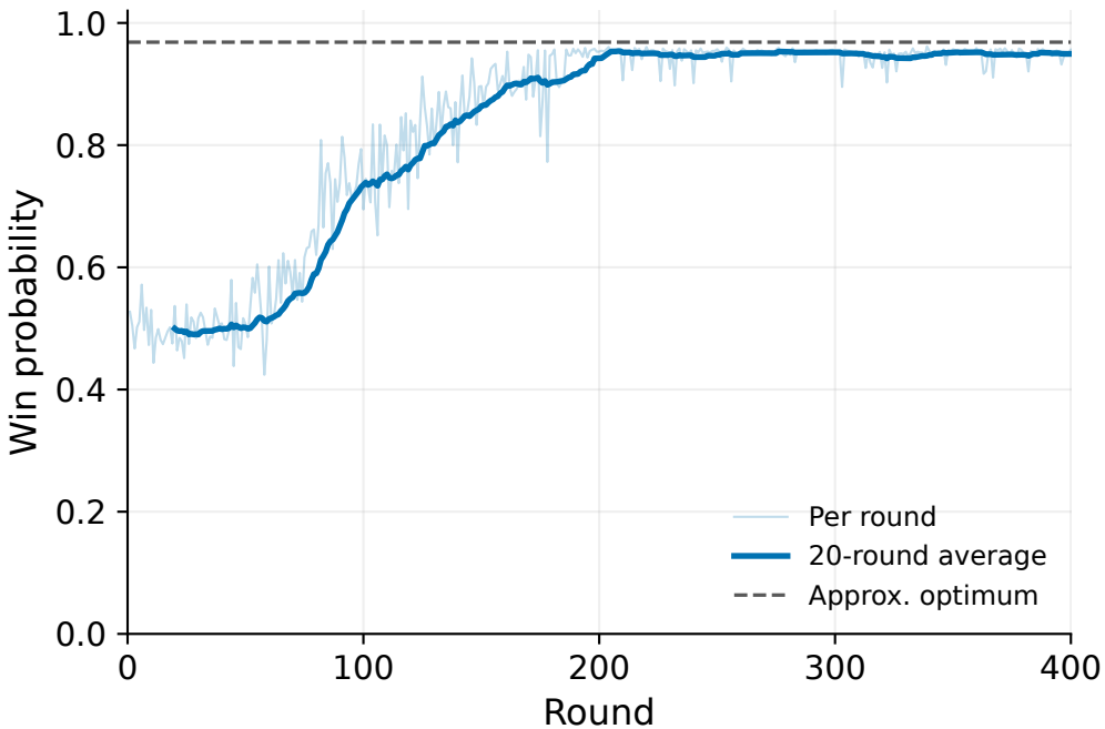
Soft Win Rate
