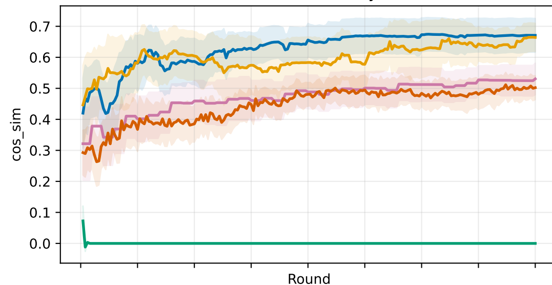
Cosine Similarity
