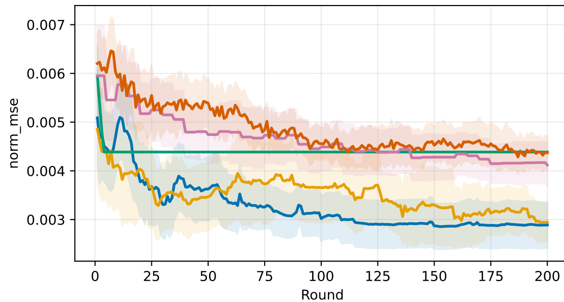
Normalized MSE
