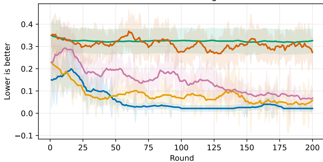
Instantaneous regret
