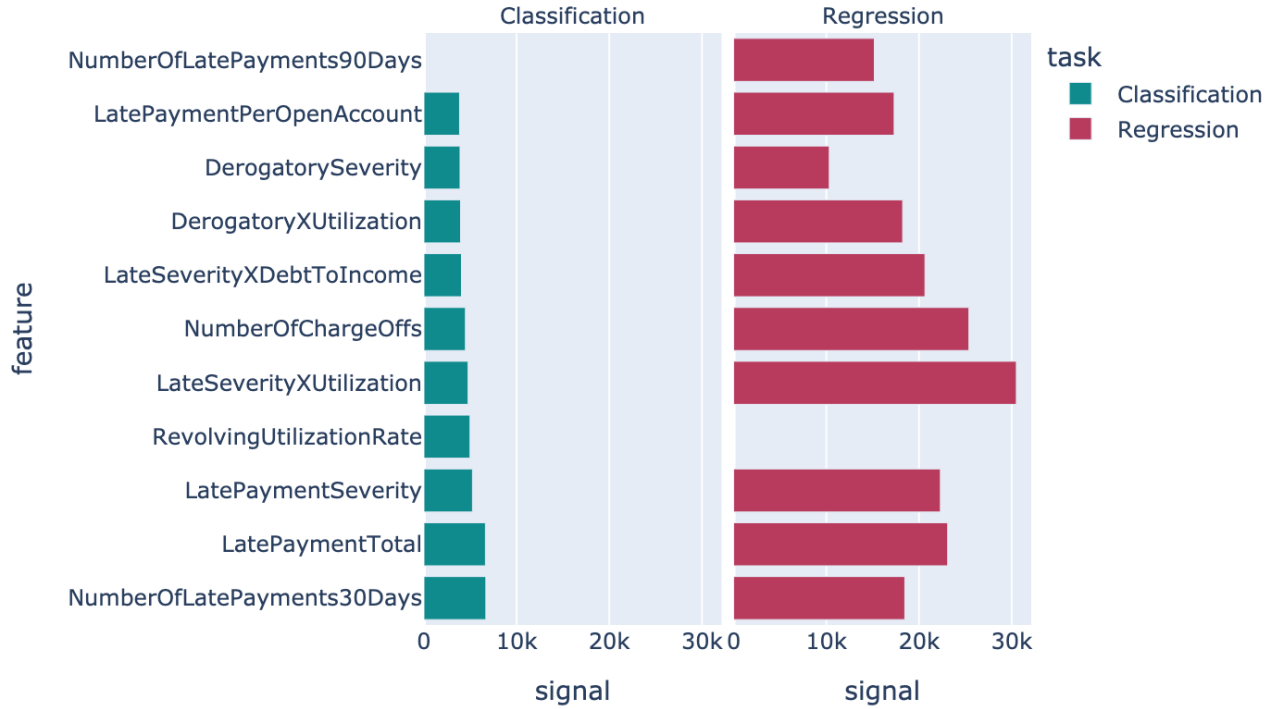
Figure 3: The strongest engineered features overlap across targets, but the ordering is not identical.
