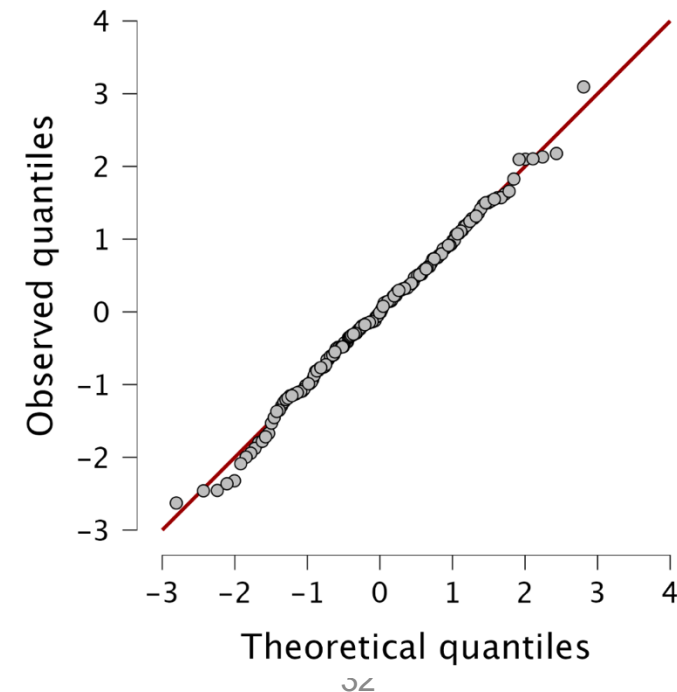
Q-Q Plot Standardized Residuals
