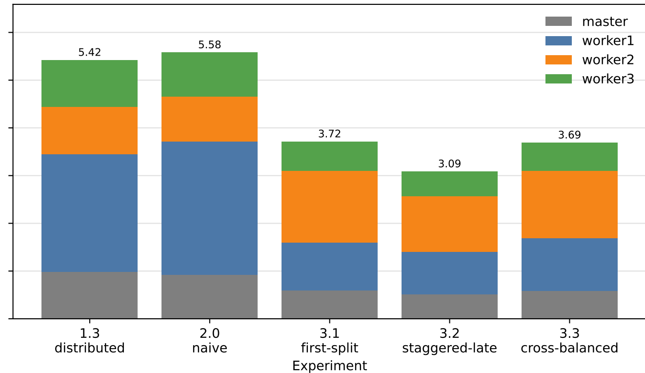
ResNet34
