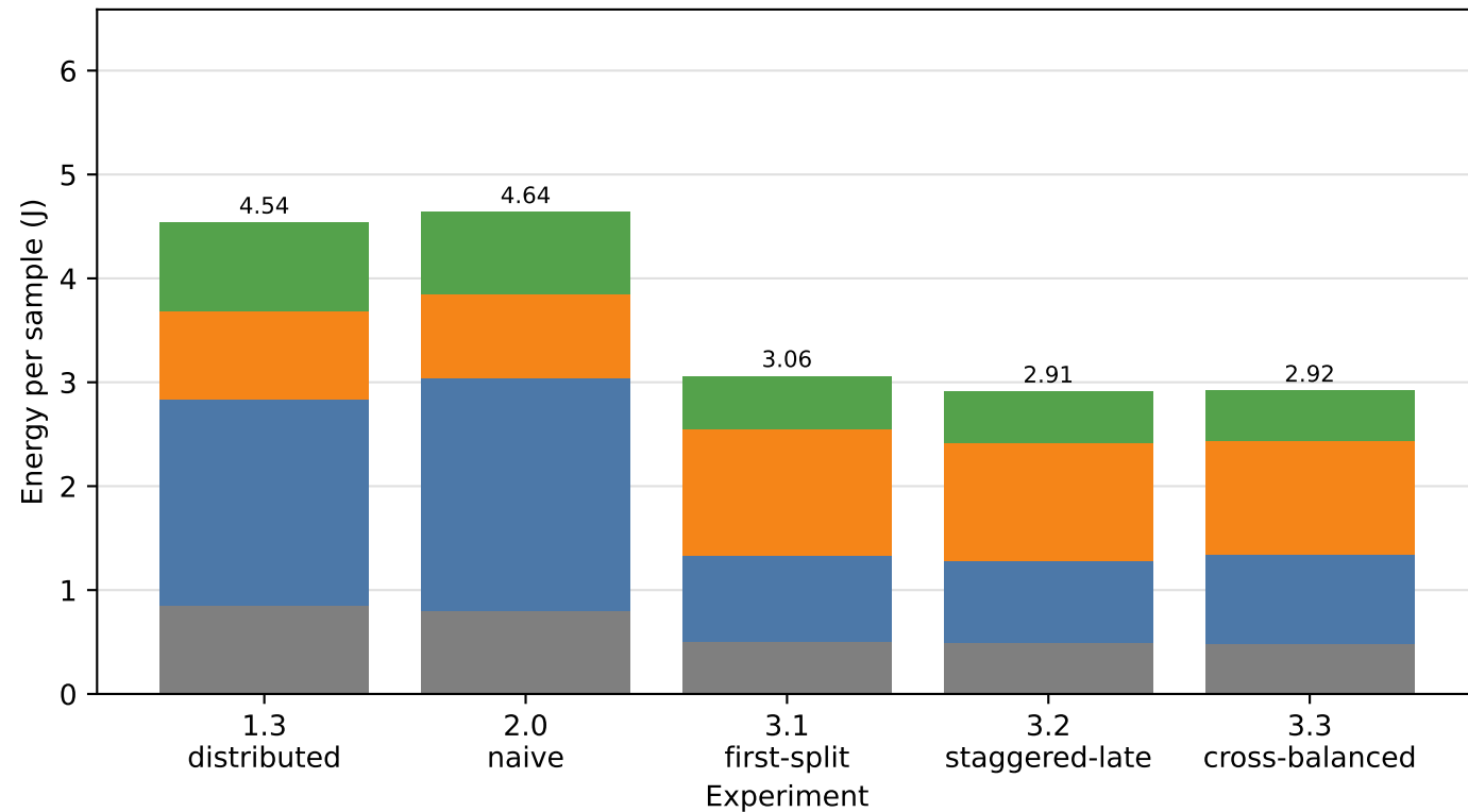
ResNet18
