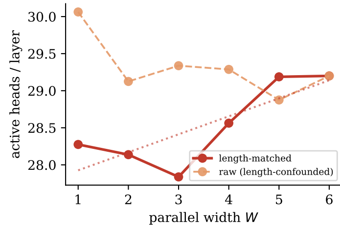
Width recruits heads r = +0.81 (length-matched)
