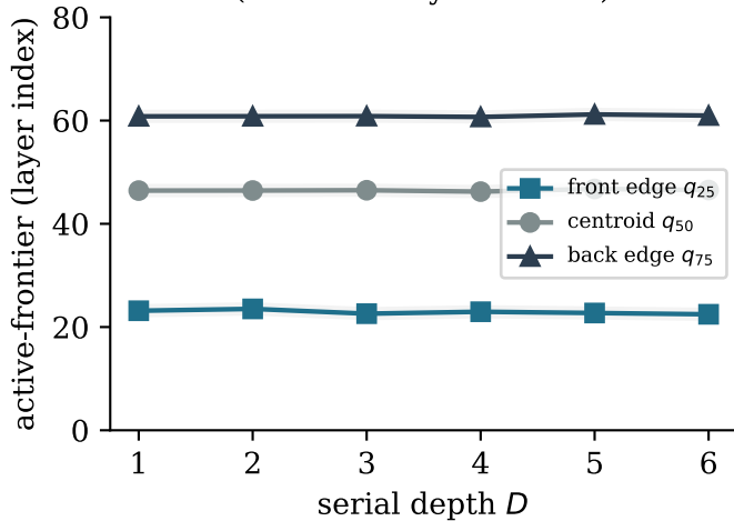
Depth: frontier flat (shifts < 1 layer = noise)
