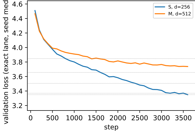
Study 1: lr 1e-3 at both widths
