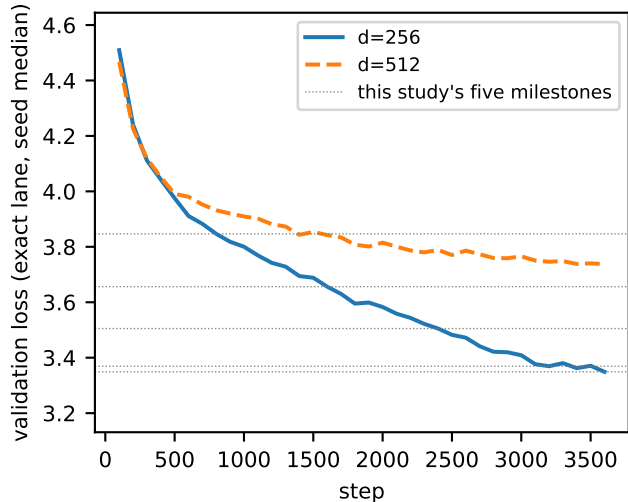
Study 1: rate 10^{-3} at both widths
