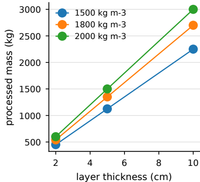
a Processed mass envelope
