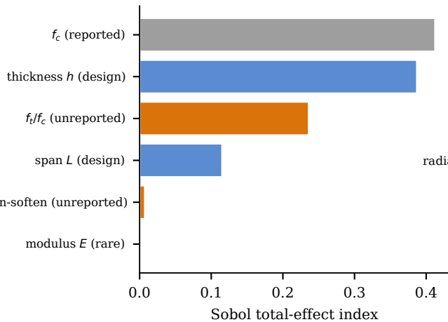
(a) Structural capacity (illustrative sensitivity runs)
