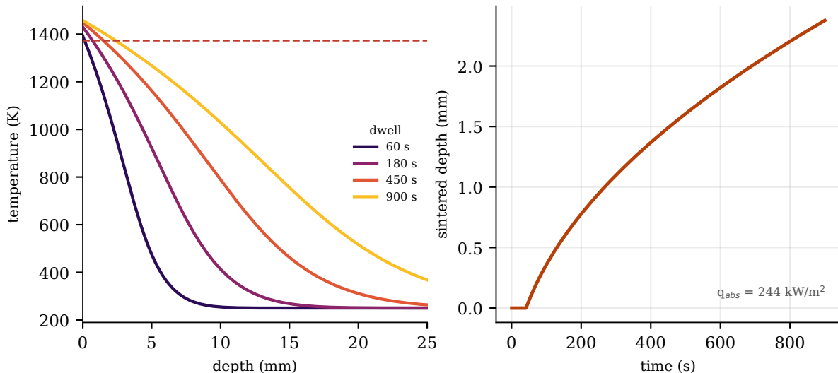
(a) Sintering is confined to a thin near-surface layer (b) Sintered depth grows slowly
