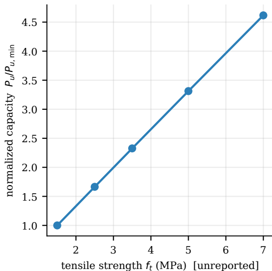
(b) At fixed reported f_c=50 MPa, capacity spans 4.6x with the unreported tensile strength
