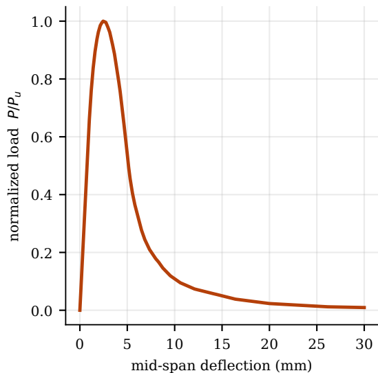
(a) Nonlinear pushover (OpenSees) sintered-regolith pad strip, f_c=50 MPa
