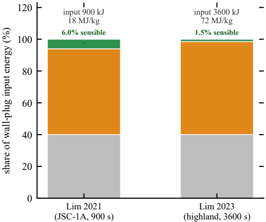
(a) Energy ledger: re-radiation dominates
