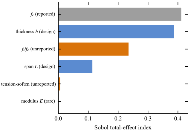
(a) Structural capacity (12,000 OpenSees pushovers)
