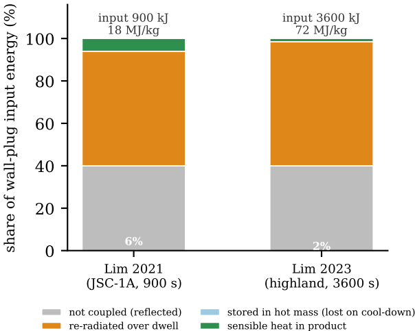
(a) Energy ledger: re-radiation dominates
