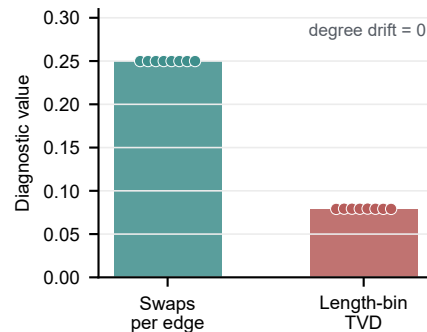
d Null diagnostics
