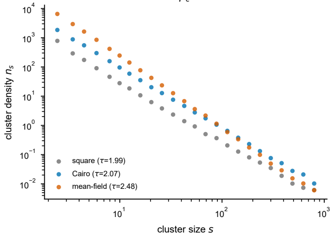
a Cluster-size distribution at p_c
