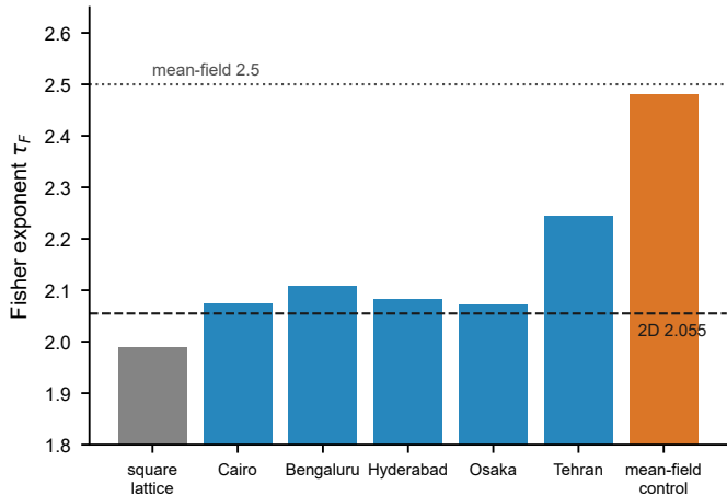
b Cluster-size-distribution exponent
