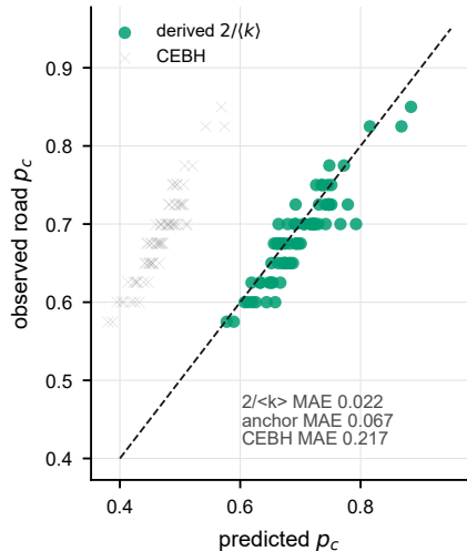
a Derived p_c = 2/\langle k \rangle (71 cities)
