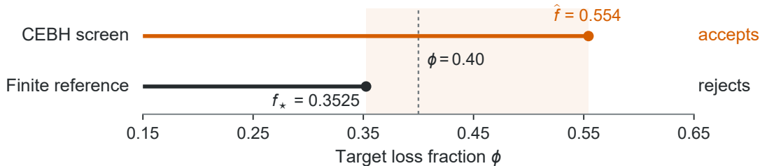
c Illustrative target on the same network
