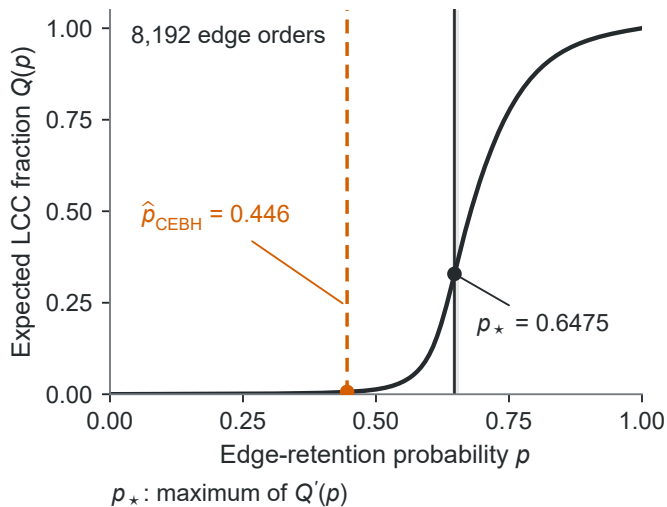
b Independent-bond response
