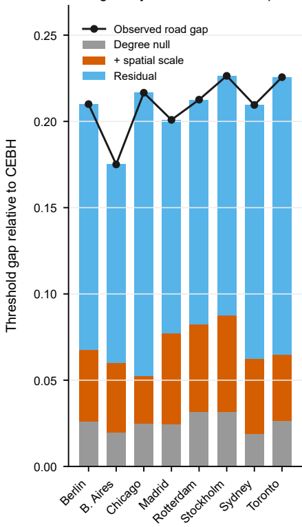
a Eight-city null-ladder decomposition
