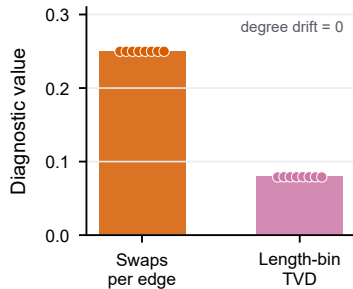
d Null-fidelity diagnostics
