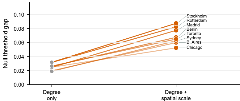
b Degree versus degree + edge-scale nulls
