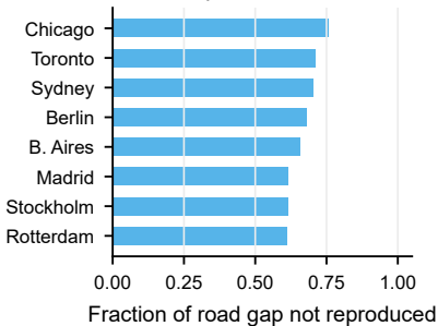
c Post-spatial residual fraction
