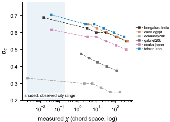
b Long-range shortcuts collapse p_c
