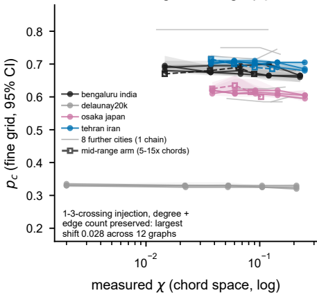
a Local/mid-range crossings: p_c bounded
