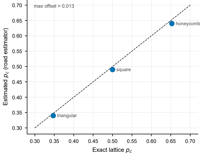
c Zero-parameter anchor (71 cities)
