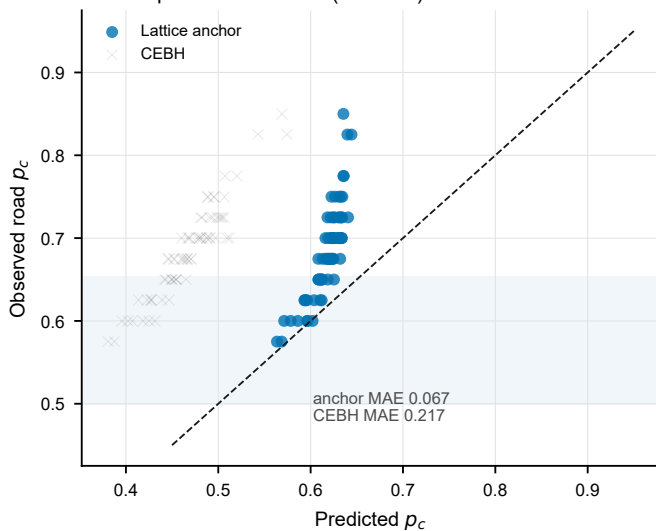
c Zero-parameter anchor (71 cities)
