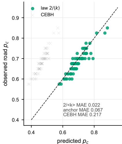
a Zero-fit p_c = 2/\langle k \rangle (71 cities)
