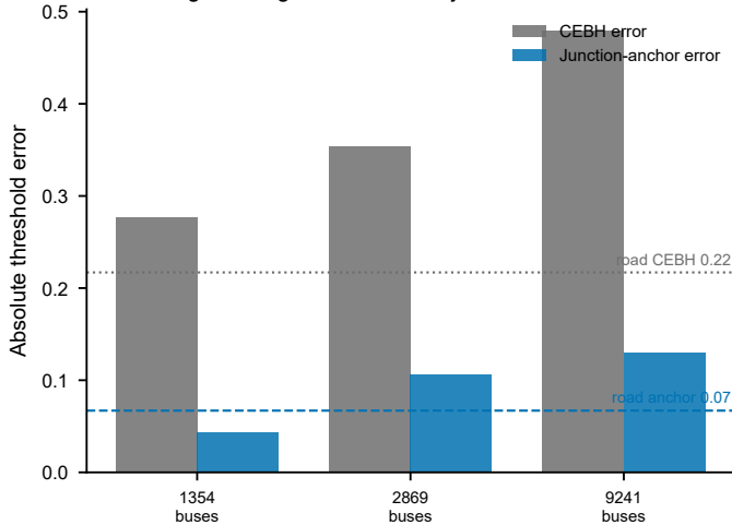
a Power grids: degree-moment vs junction anchor
